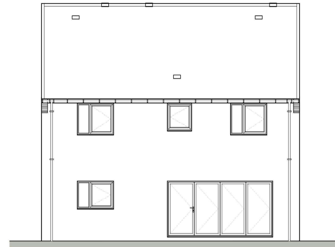
SIDE ELEVATION
